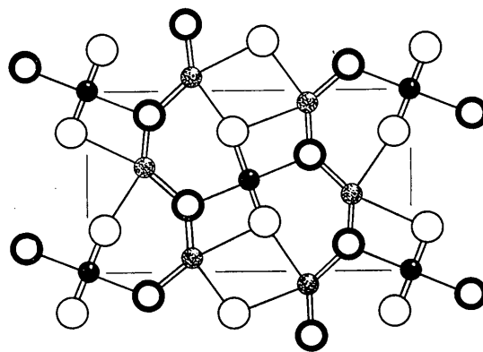
Fig. 2. The structure of Mn_2GeO_4 in projection on to (001). Small black circles Ge; stippled circles Mn; largest circles oxygen appearing at two levels.
